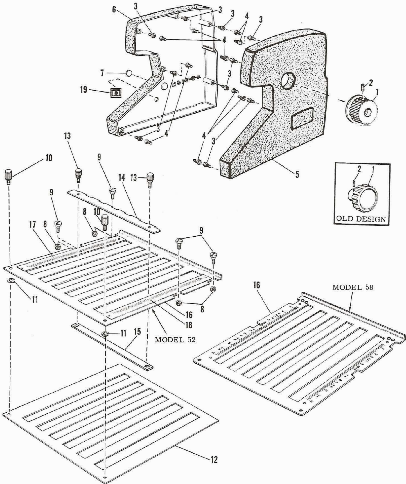
FIGURE 1 — MODELS 52-58 Side Covers, First Fold Plate
