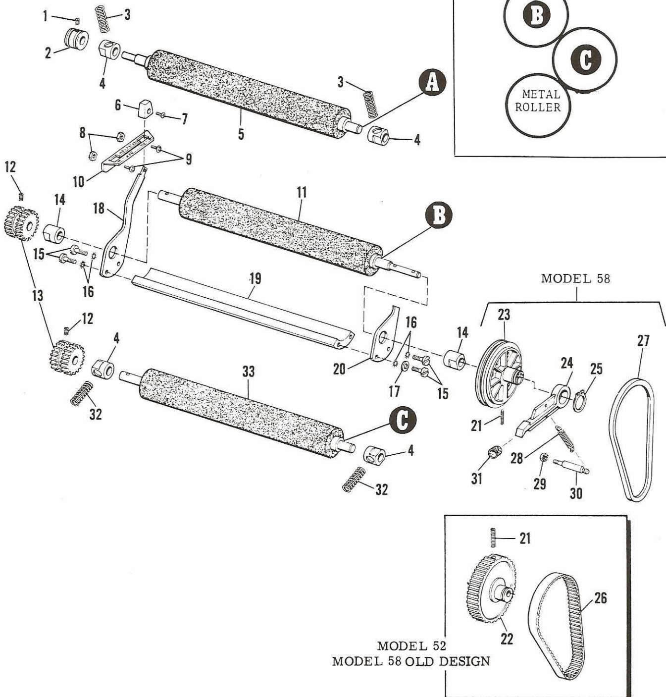
FIGURE 5 – MODELS 52-58 Folder Rollers and Deflector Mechanism
